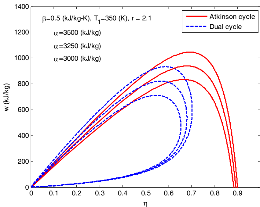
Figure 3 Effect of \alpha on the w versus \eta characteristics.
